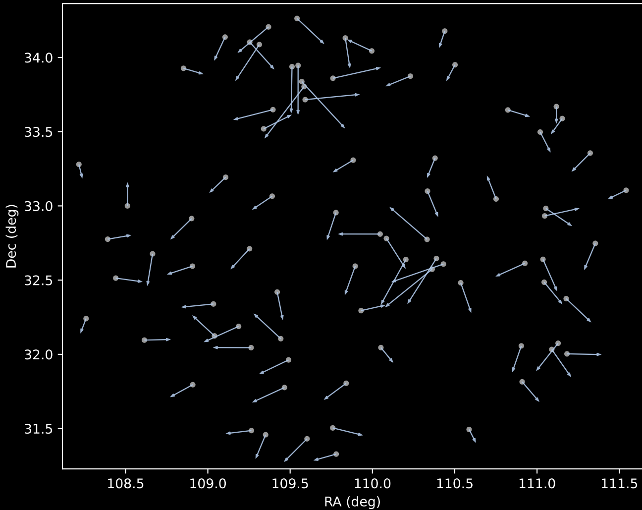
APOGEE DR17 Cluster 1 Proper Motion Vectors (n=81)
