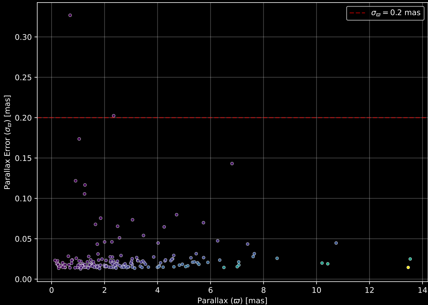
APOGEE DR17 Field: [120-30] Parallax Quality (n= 191)
