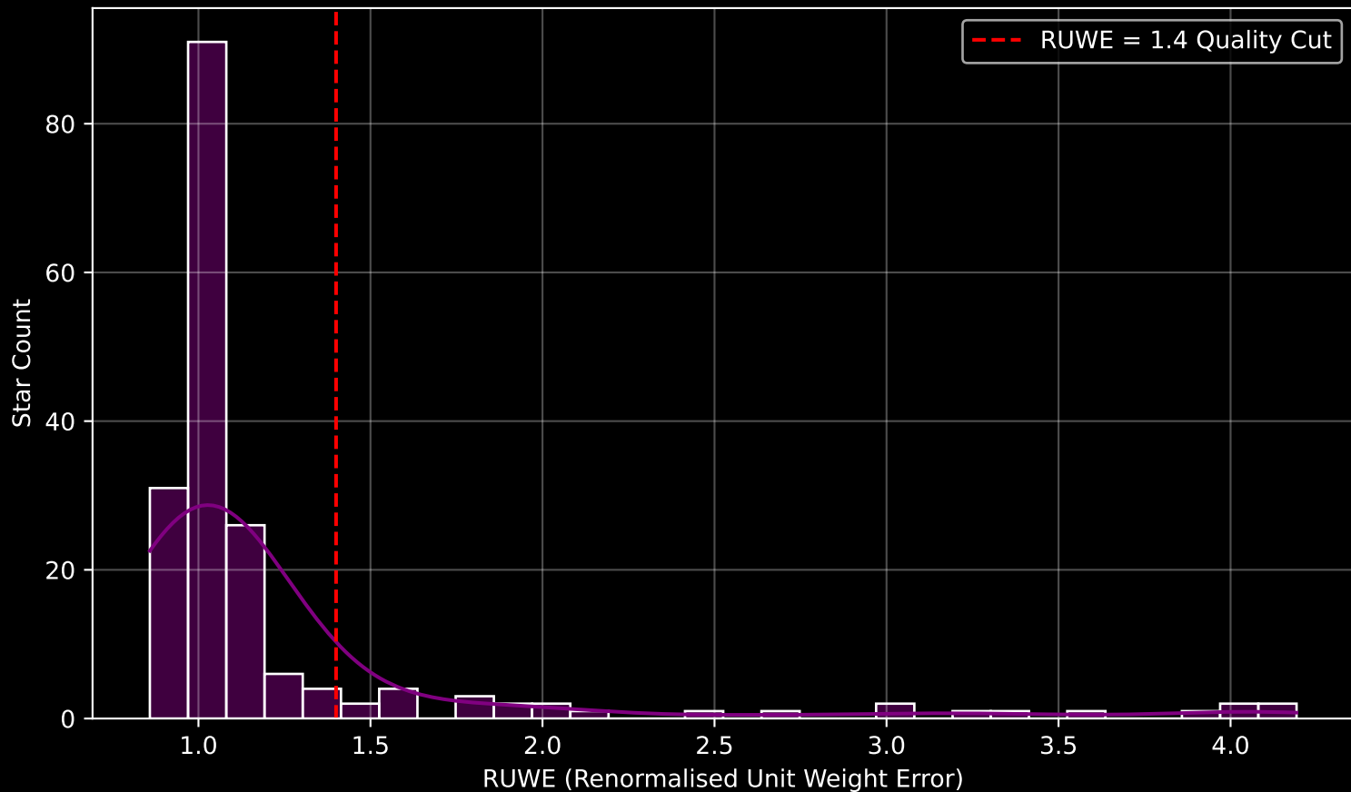
GAPOGEE DR17 Field [120-30] RUWE Distribution (n= 184)
