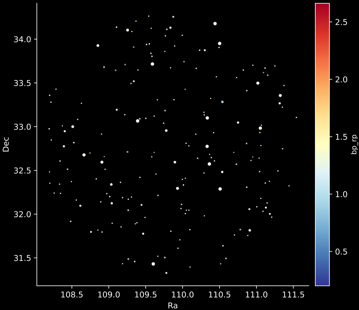
APOGEE DR17 Field: [120-30] Stars: 191
