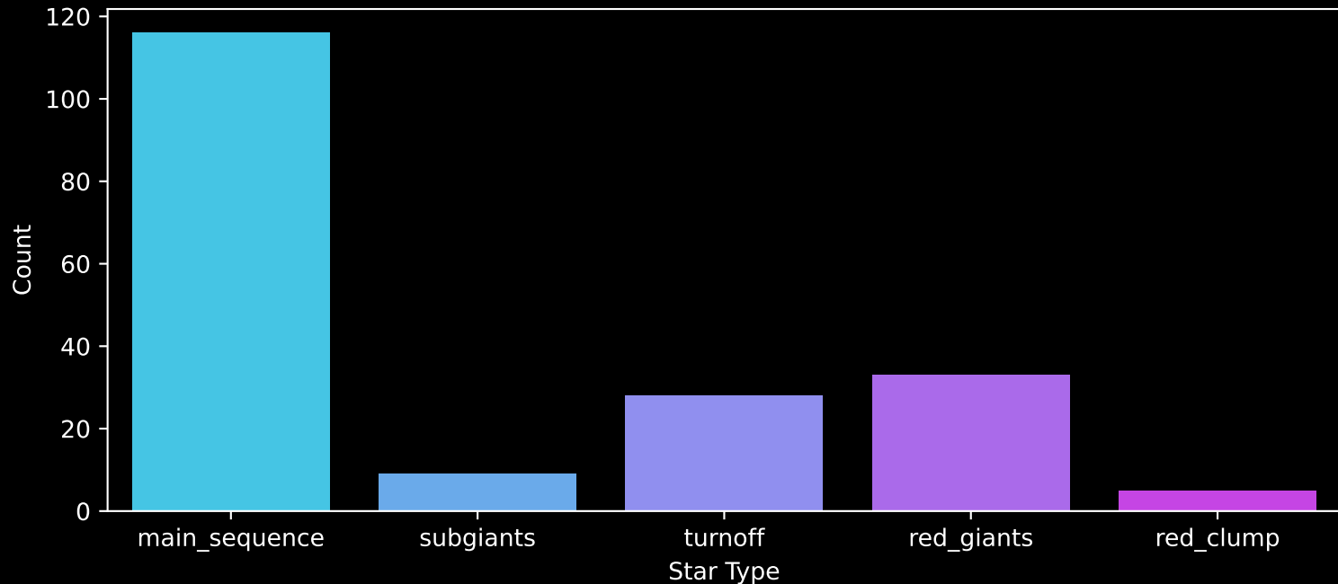
APOGEE DR17 Field: [120-30] Count plot of Star Type
