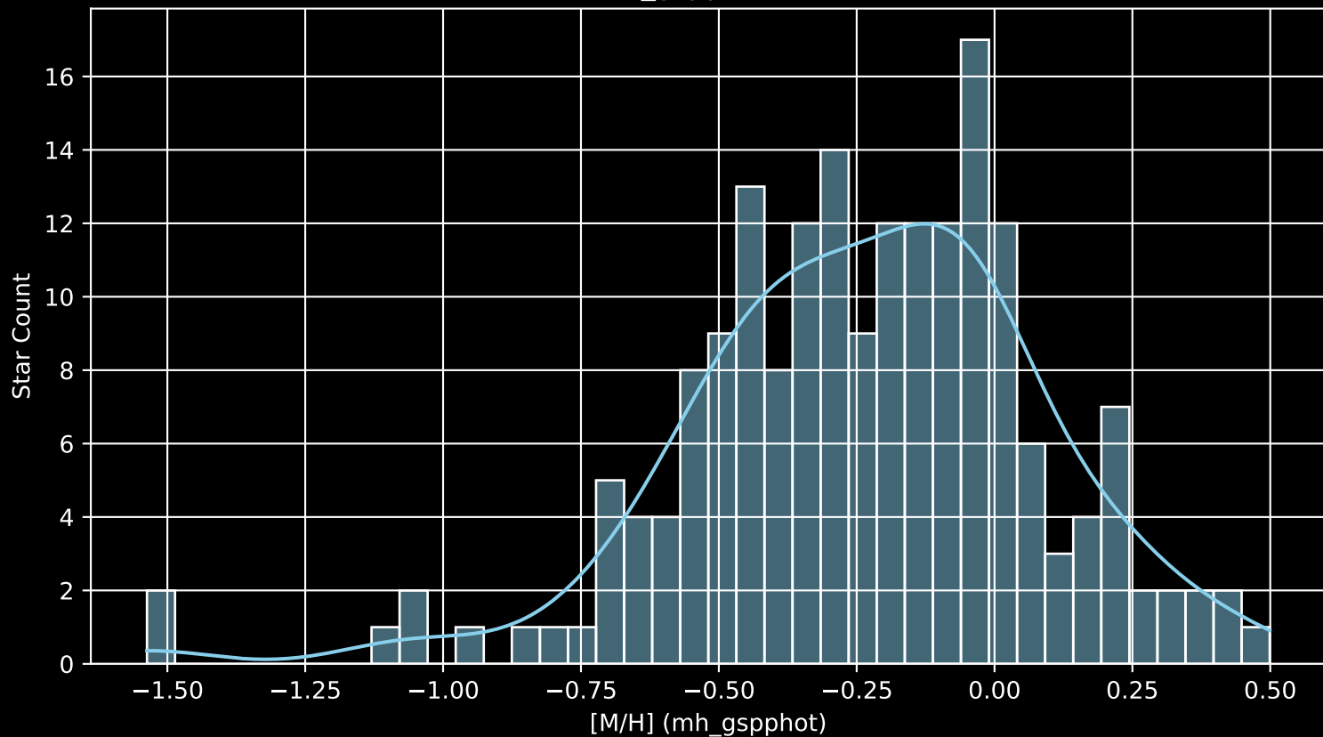
APOGEE DR17 Field: [120-30 [M/H] (mh_gspphot) (n= 189)
