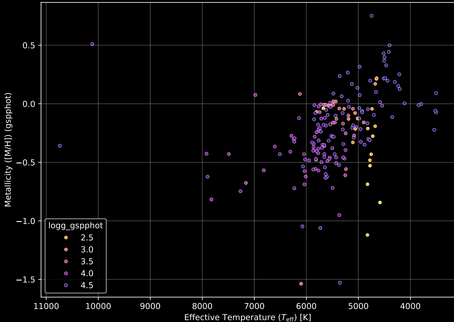
APOGEE DR17 Field: [120-30] Stellar Population Parameters (n= 191)
