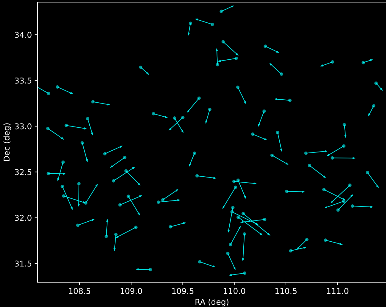
APOGEE DR17 Noise Stream Proper Motion Vectors (n=81)
