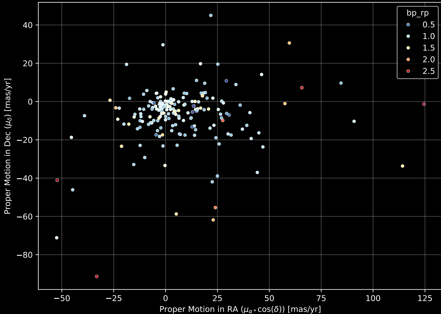
APOGEE DR17 Field: [120-30] Proper Motion Diagram (n= 191)
